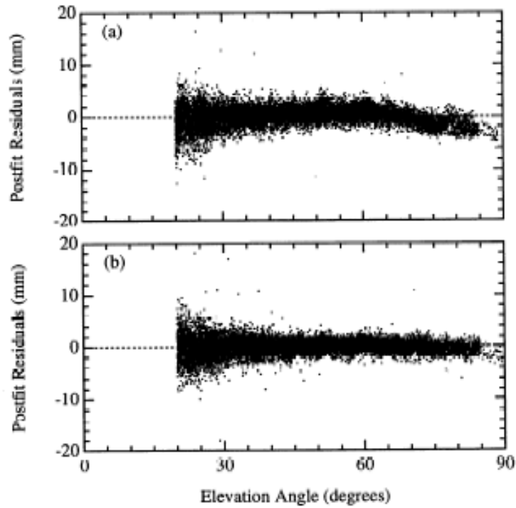
Left: Phase residuals versus elevation for Westford pillar, without (top) and with (bottom) microwave absorber.
